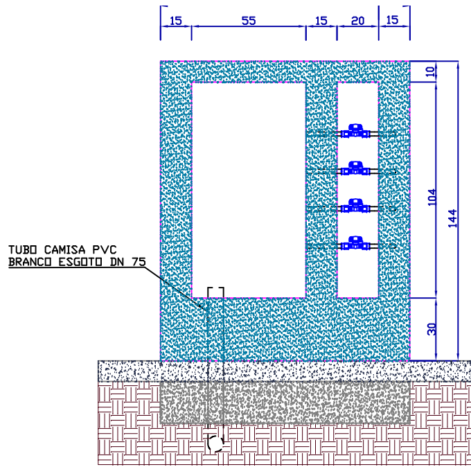
VISTA FRONTAL
